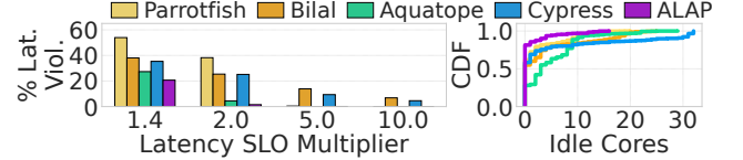
Figure 14: ALAP is robust to a range of SLOs, providing the lowest violations while minimizing resource waste. See § 9.5.
