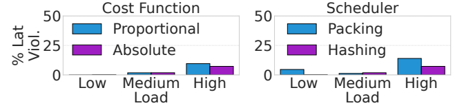
Figure 7: Design exploration of ALAP's (a) cost function and (b) scheduler algorithm. ALAP incurs fewer SLO violations using the absolute cost function in its Resource Allocator and a hashing -based scheme in its Scheduler. See § 5.3 & 6.
