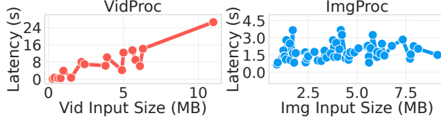
Figure 2: Contrary to the assumption of previous works, many common serverless functions do not exhibit linear relationships between size and execution time. See § 2.
