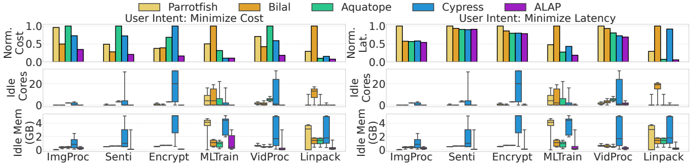
Figure 9: ALAP reduces cost and resource waste for all functions. It considerably reduces latency for multi-threaded functions without harming single-threaded functions. Values per function show the max. See § 9.1.2.
