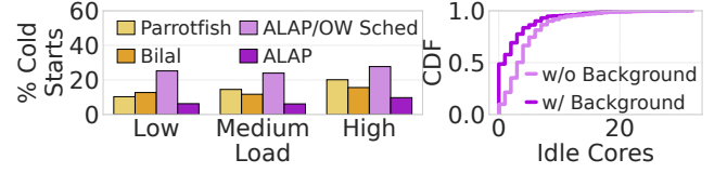
Figure 13: ALAP’s Scheduler reduces (a) cold starts by using warm, predicted-sized or larger containers (left) and (b) resource waste by provisioning right-sized containers in the background (right). See § 9.4.
